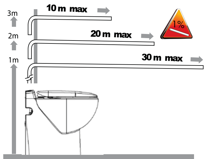
SANICOMPACT® 48 SILENCE ECO+ code: C48
